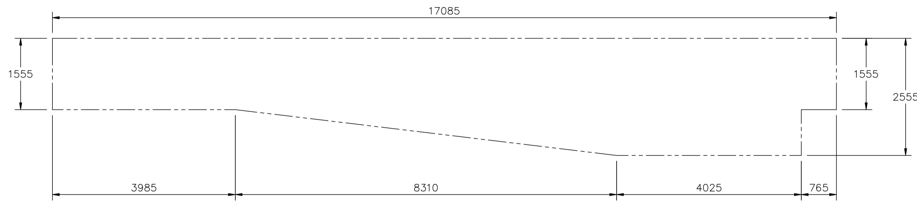
EXCAVATION DETAILS
