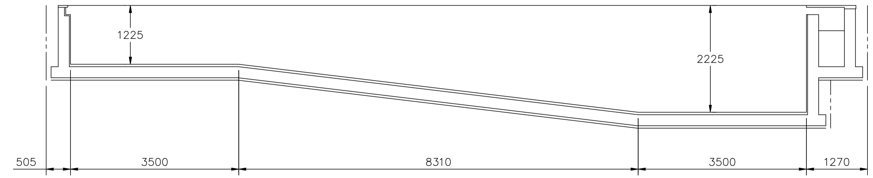
SECTION THRO' POOL
